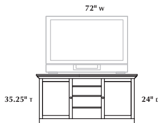
RC-3572 • WC-3572 (35.25" tall) RC-2472 • WC-2472 (24" tall)
